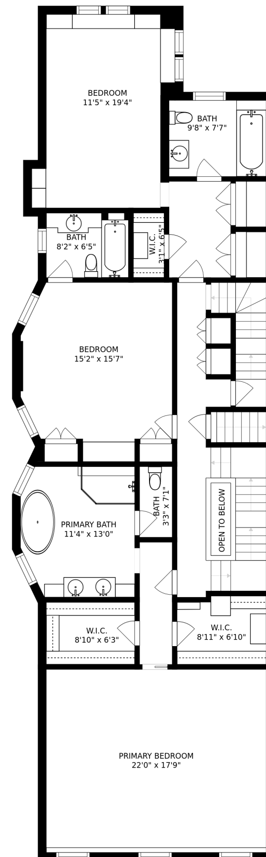
FLOOR 3
