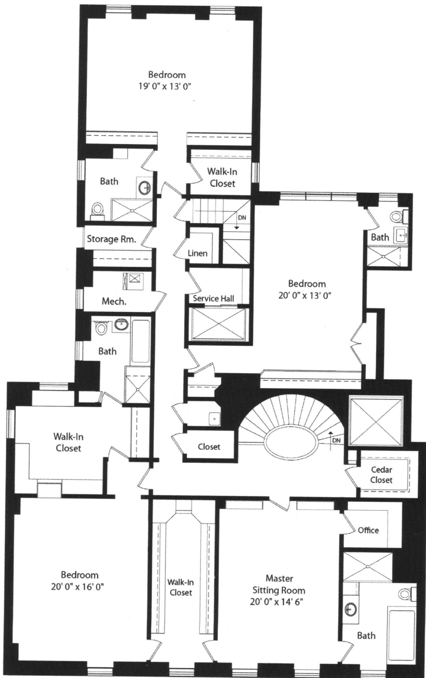
Second Floor
