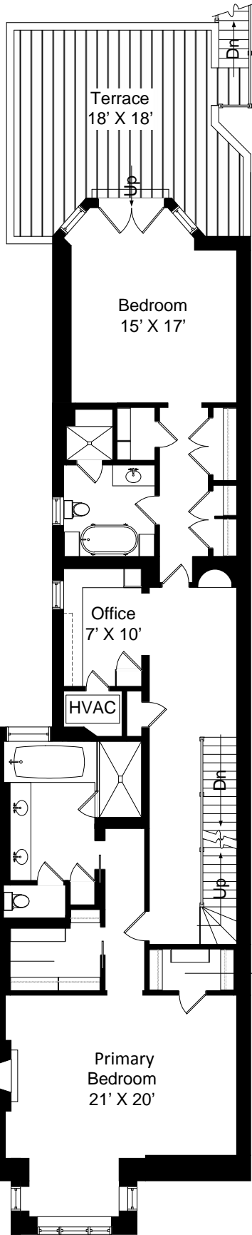
SECOND LEVEL
