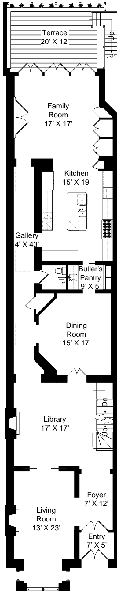
MAIN LEVEL
